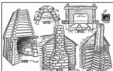
Source: Stick Chimney - Detail for fireplaces and flues
